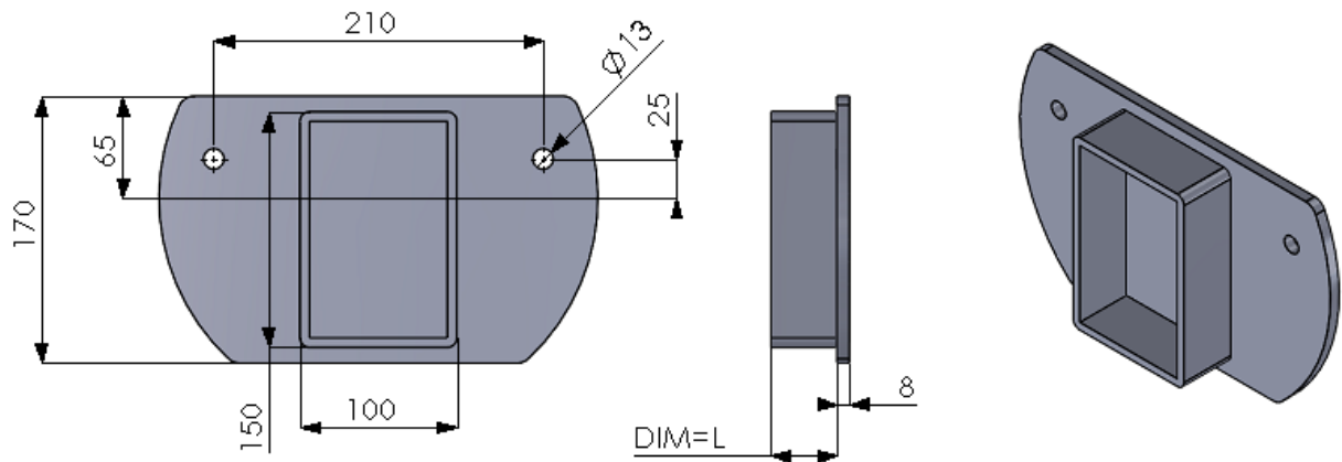
31642 Pedestal L=42mm (Total 50mm) 31643 Pedestal L=22mm (Total 30mm)
