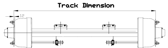
* Axle Track Dimension
